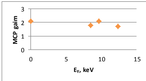
Figure 5: Dependence of MCP2 gain on photon energy at increase of MCP voltage from 1.8 kV to 1.85 kV.
