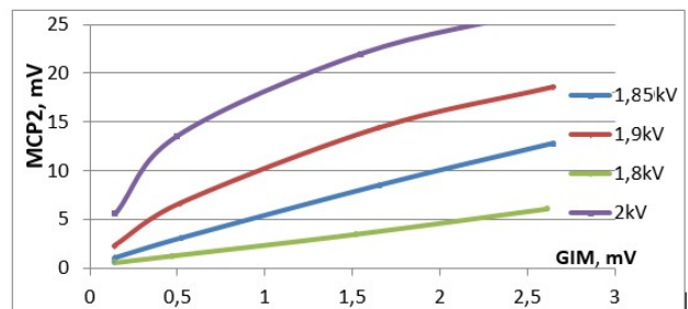
Figure 4: Dependence of MCP2 signal on gas ionization chamber signal at different MCP 2 voltages.
