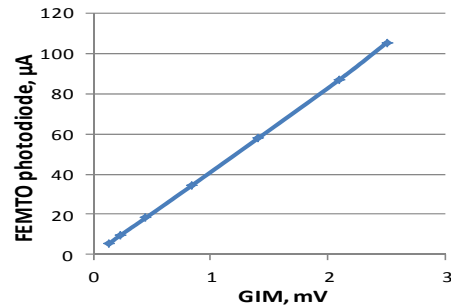
Figure 6: Dependence of XFEL Canberra PIPS diode current on gas ionisation monitor (GIM) signal at E_\gamma=9.66 keV.
