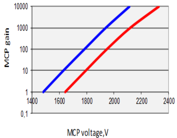
Figure 3: Dependence of MCP1 (blue line) and MCP2 (red line) gains on MCP voltage.
